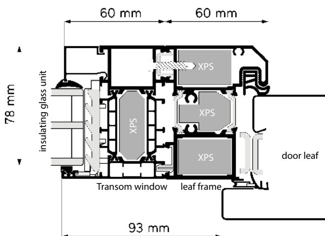
Cross section of Aluthermo Comfort 73+ doors with a side transom window
